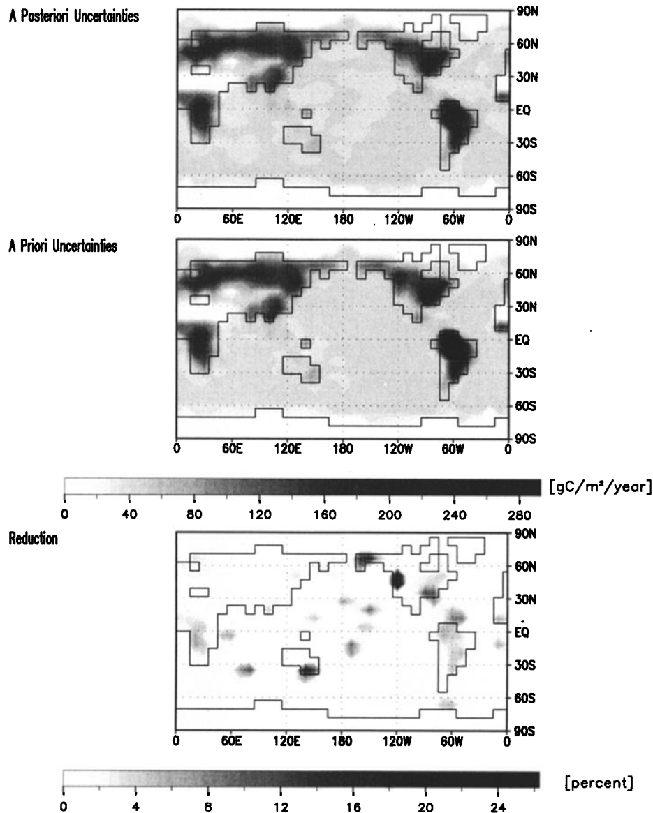
Figure 10. A priori and a posteriori uncertainties for the annual mean of the sum of the biospheric and oceanic flux components and the difference of their quotient from 1 in percent. Values close to 100 quantify small posterior uncertainty.
