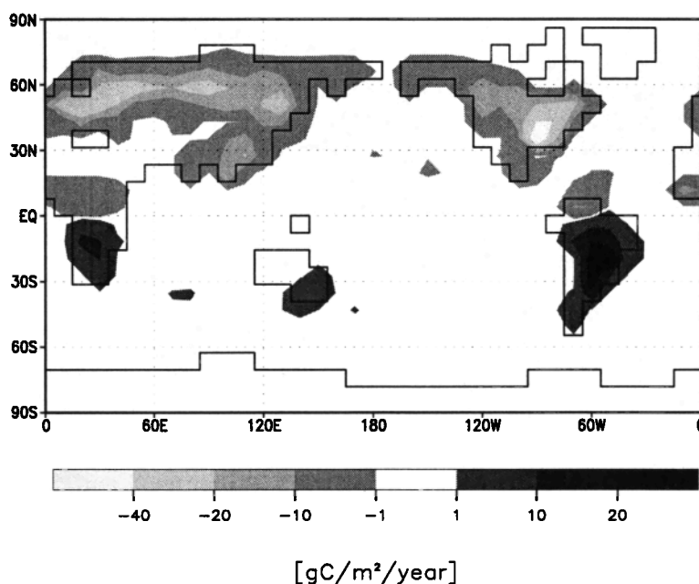
Figure 6. Annual mean fluxes computed from the second right-hand singular vector.
