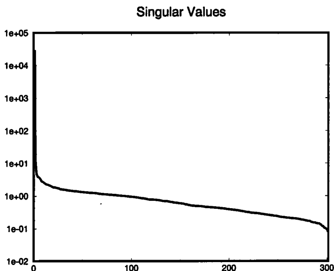
Figure 5. Spectrum of singular values.
