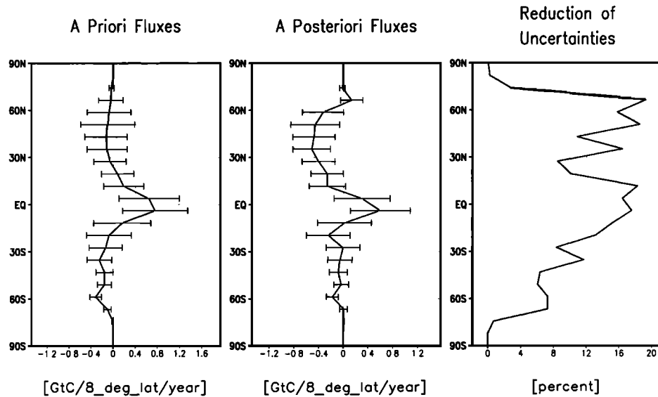
Figure 8. A priori and a posteriori uncertainties for the zonal and annual mean of the sum of the biospheric and oceanic flux components and the difference of their quotient from 1 in percent. Values close to 100 quantify small posterior uncertainty.
